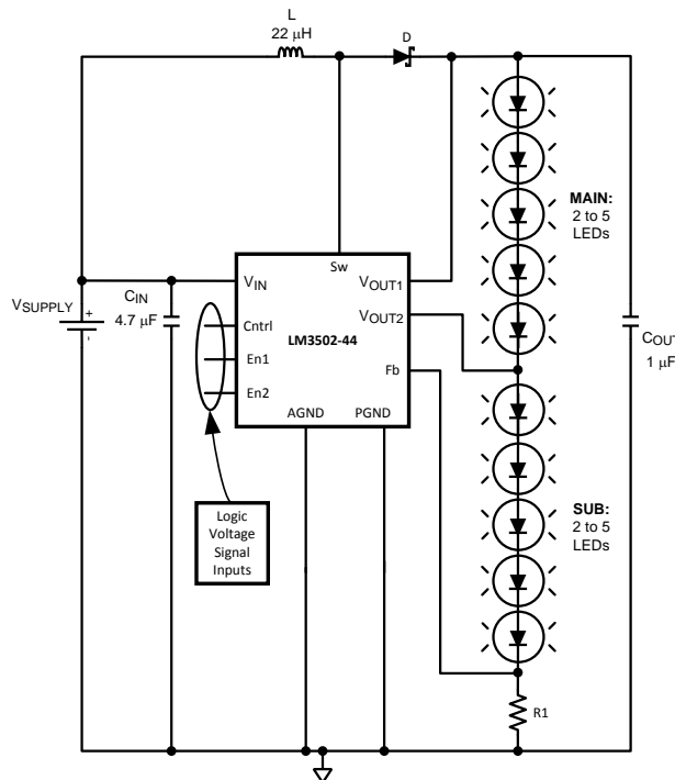
Figure 1. Backlight Configuration with 10 White LEDs
